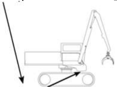
Maximum clearance between the top of the steel shoe and the body/attachment of the machine
